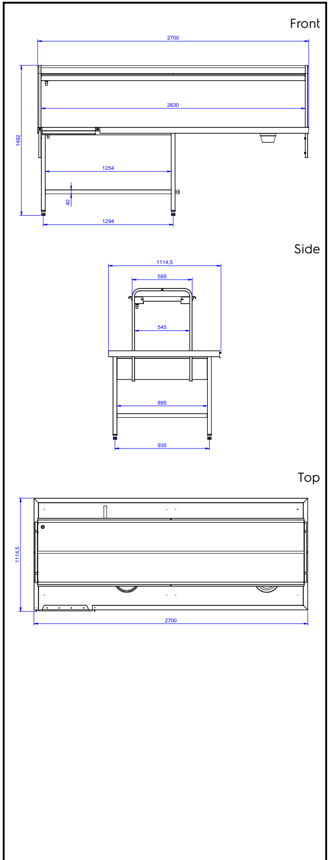
Handling System Sorting Table Right to Left, 2700x1100mm
